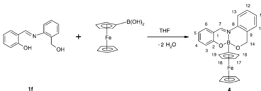
Scheme 3. Monomeric boron compound from an aromatic tridentate ligand
