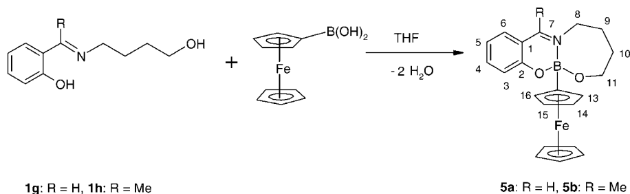
Scheme 4. Monomeric boron compounds from tridentate ligands derived from 4-aminobutanol
