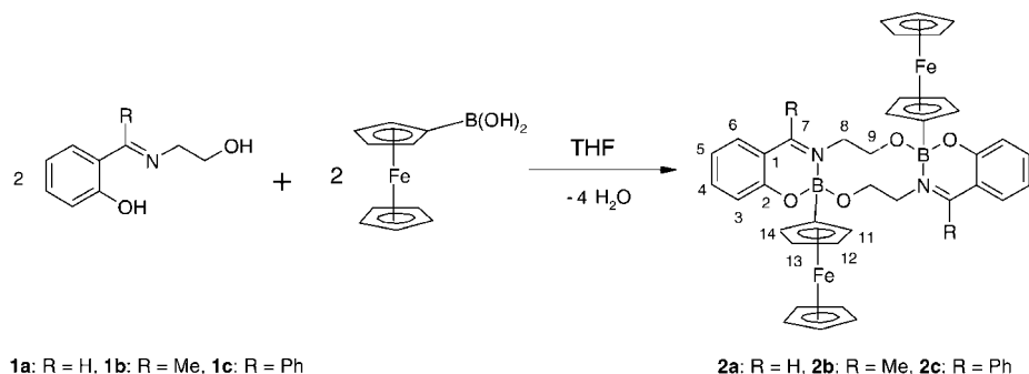
Scheme 1. Dimeric boron compounds from tridentate ligands
