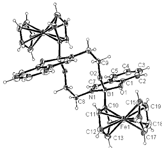
Figure 1. Molecular structure of solid-state 2a
