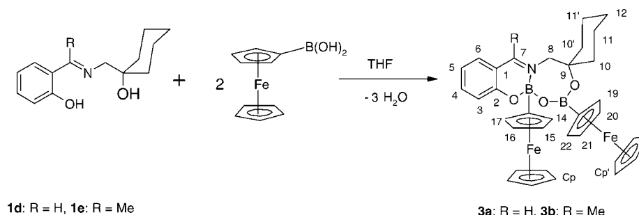
Scheme 2. Boron complexes having two boron atoms with different geometry
