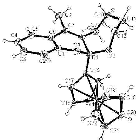
Figure 2. Molecular structure of solid-state 5b
